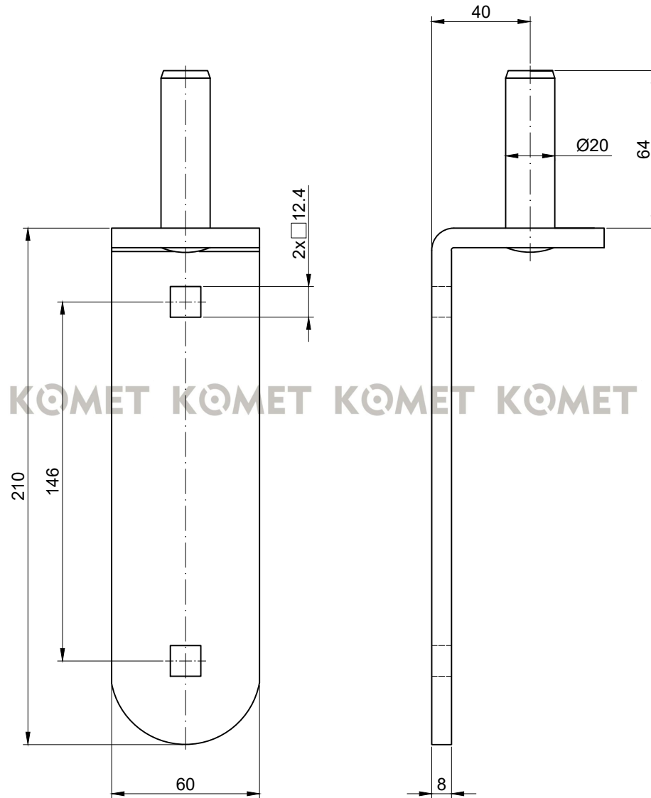
KOMET Pintle Ø 20 to L-1150 for screwing
