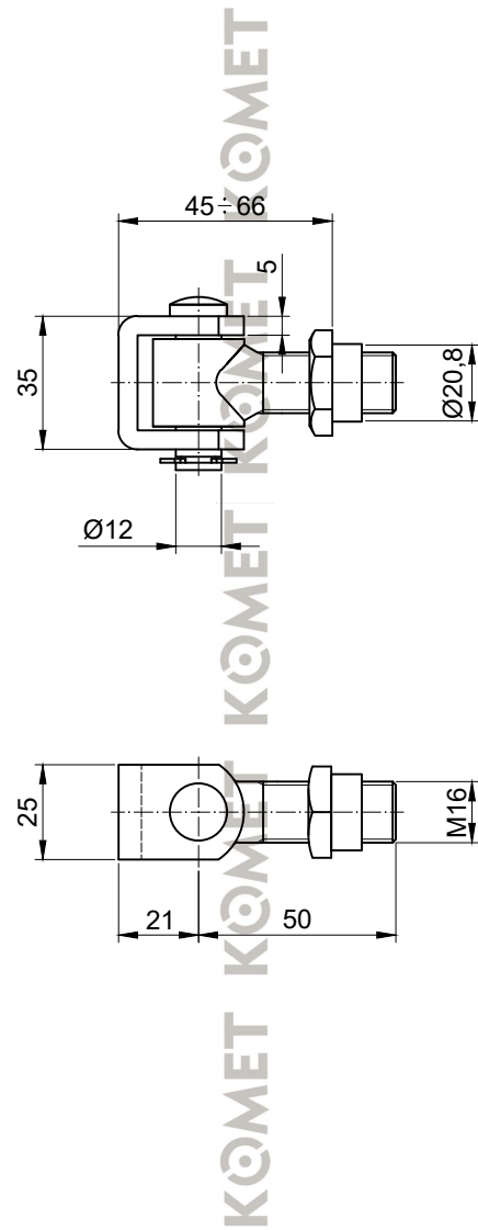
KOMET Adjustable hinge M16 with a bush, welded
