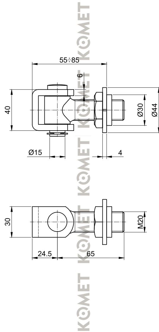
KOMET Adjustable hinge M20 welded
