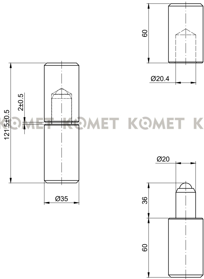
KOMET Turned hinge \varnothing 35 with a ball
